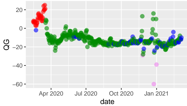
Pima tseries, 2021-03-10 - hc complete
