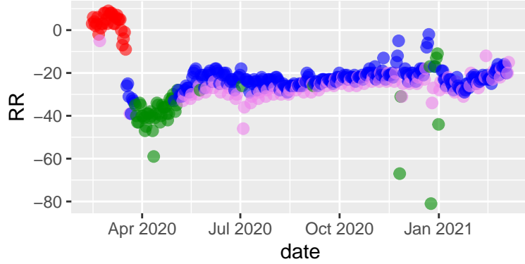
Pima tseries, 2021-03-10 - rpart
