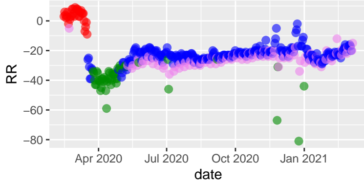
Pima tseries, 2021-03-10 - kmeans
