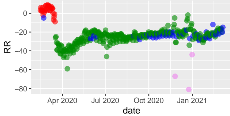
Pima tseries, 2021-03-10 - hc complete
