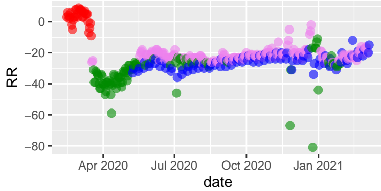
Pima tseries, 2021-03-10 - fanny
