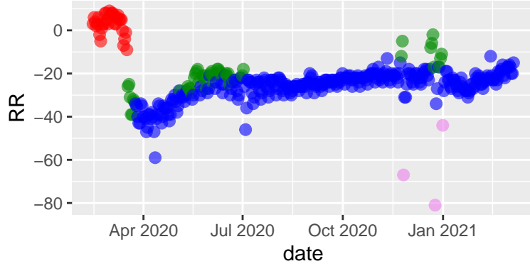
Pima tseries, 2021-03-10 - diana
