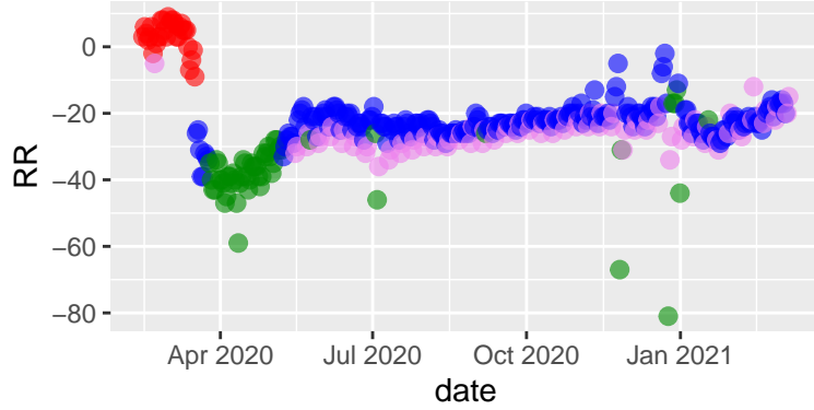
Pima tseries, 2021-03-10 - agnes
