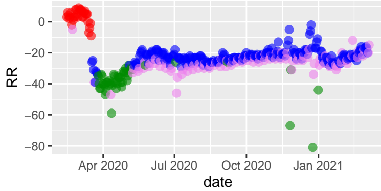
Pima tseries, 2021-03-10 - xgb
