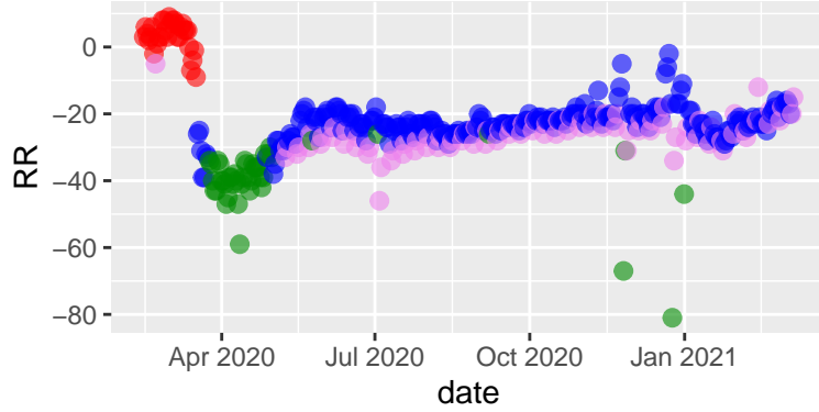
Pima tseries, 2021-03-10 - clara
