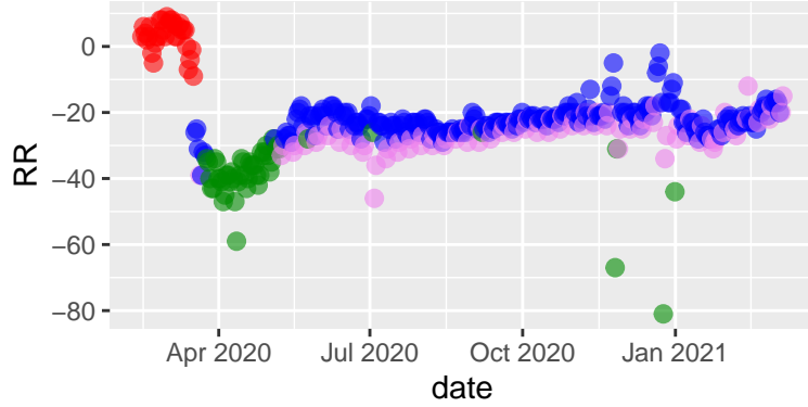
Pima tseries, 2021-03-10 - rf
