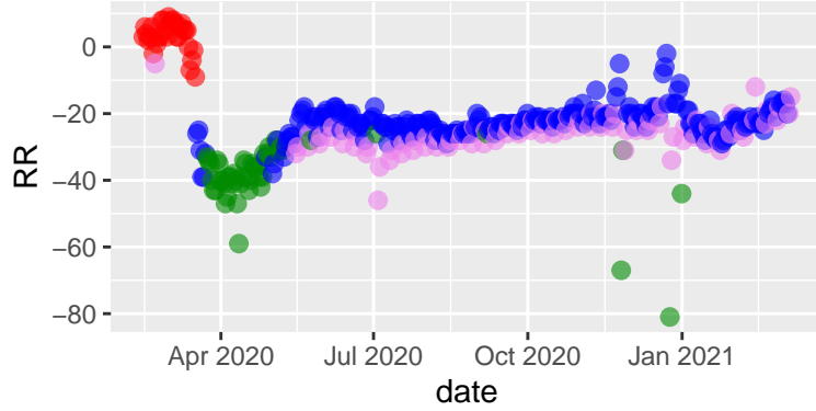
Pima tseries, 2021-03-10 - pam
