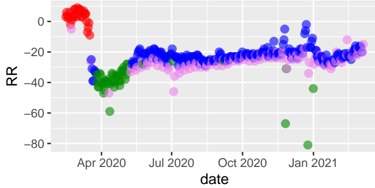
Pima tseries, 2021-03-10 - hc Ward
