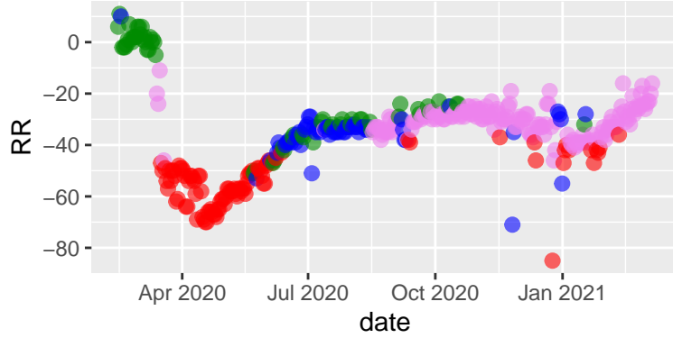
Marin tseries, 2021-03-10 - xgb
