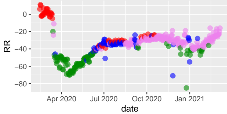
Marin tseries, 2021-03-10 - rpart
