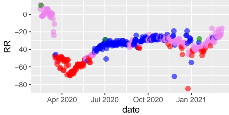
Marin tseries, 2021-03-10 - hc complete
