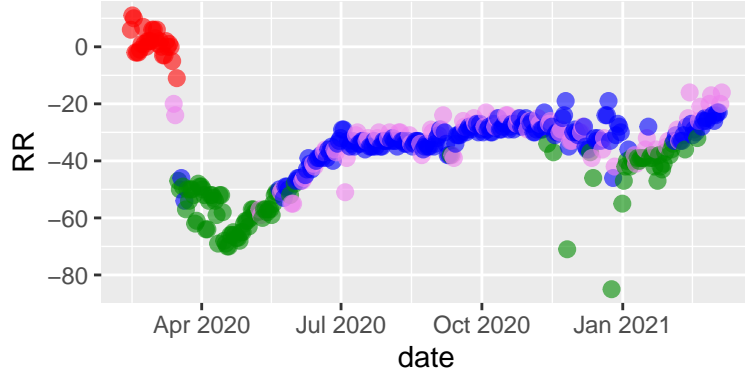
Marin tseries, 2021-03-10 - kmeans
