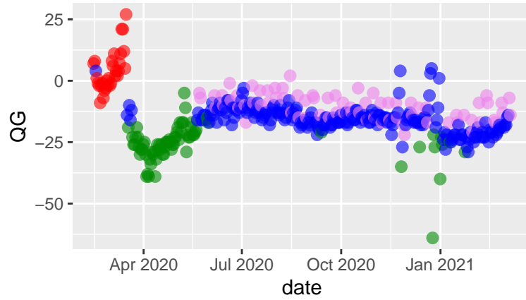
Marin tseries 2021-03-10 - agnes agnes
