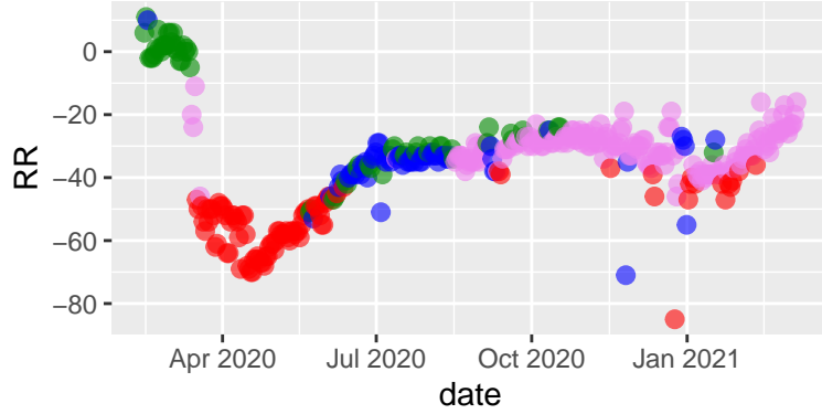
Marin tseries, 2021-03-10 - hc Ward
