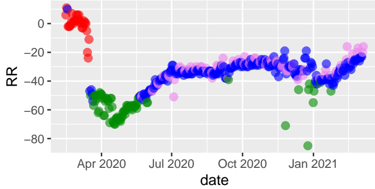
Marin tseries 2021-03-10 - agnes agnes
