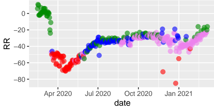
Marin tseries 2021-03-10 - clara
