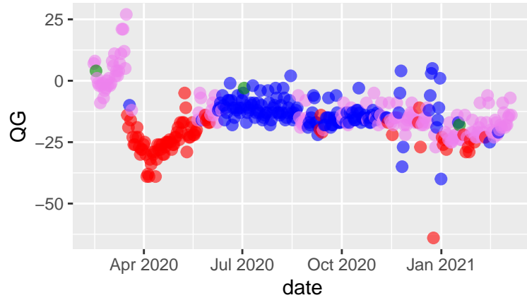
Marin tseries, 2021-03-10 - hc complete
