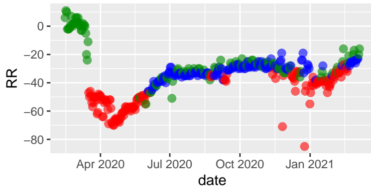
Marin tseries 2021-03-10 - fanny
