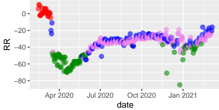
Marin tseries, 2021-03-10 - pam
